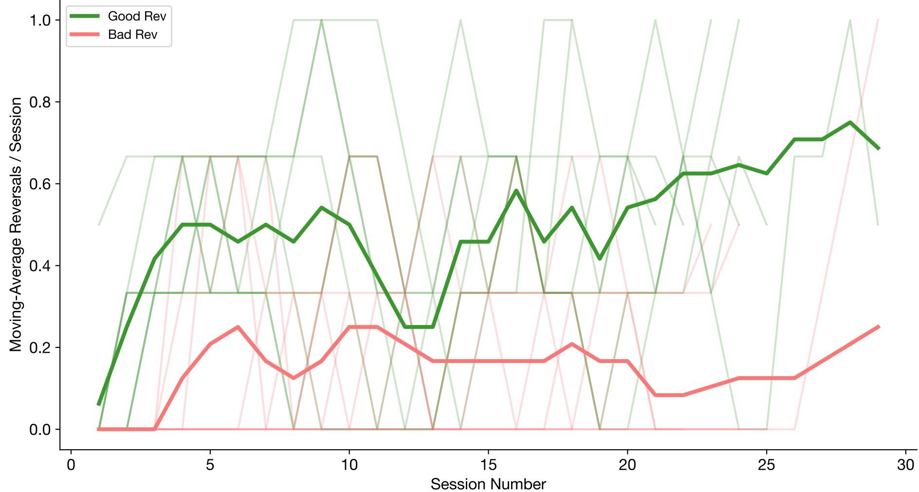
Moving-Average Good and Bad Reversals Over Time (n=8 subjects; sessions per subject=18–29; window=3)
